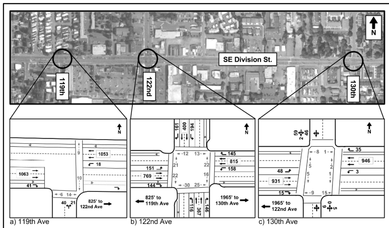
Figure 3.3 Intersection Volumes
